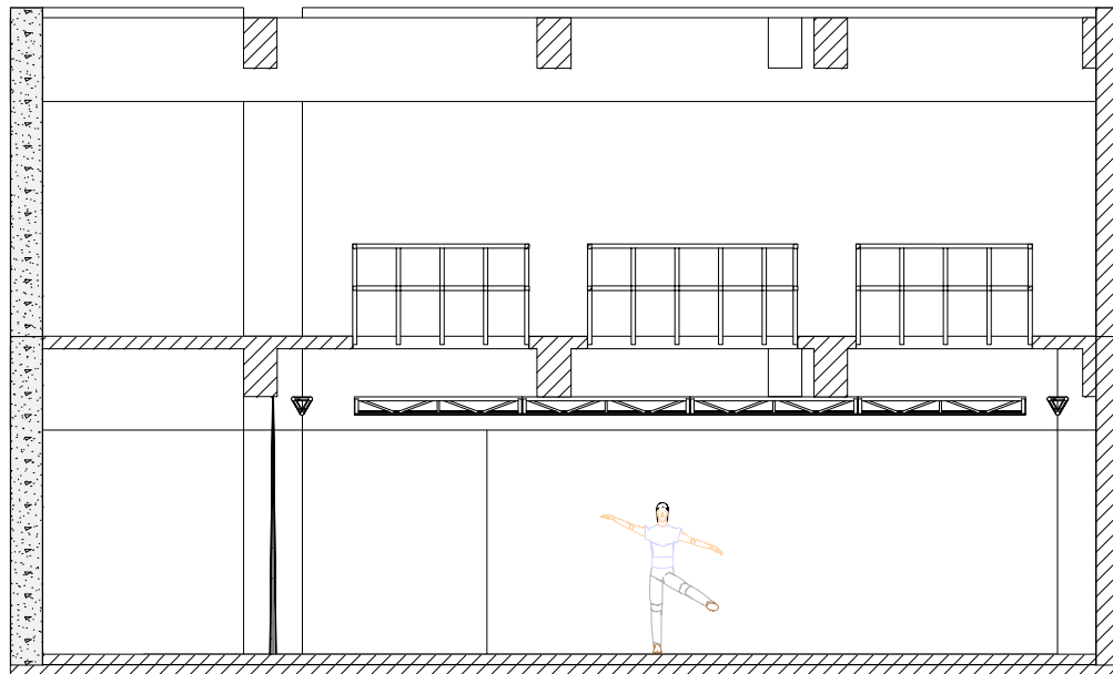
Cross Section
